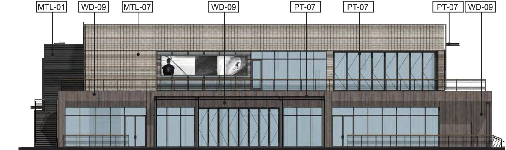
SOUTH ELEVATION
