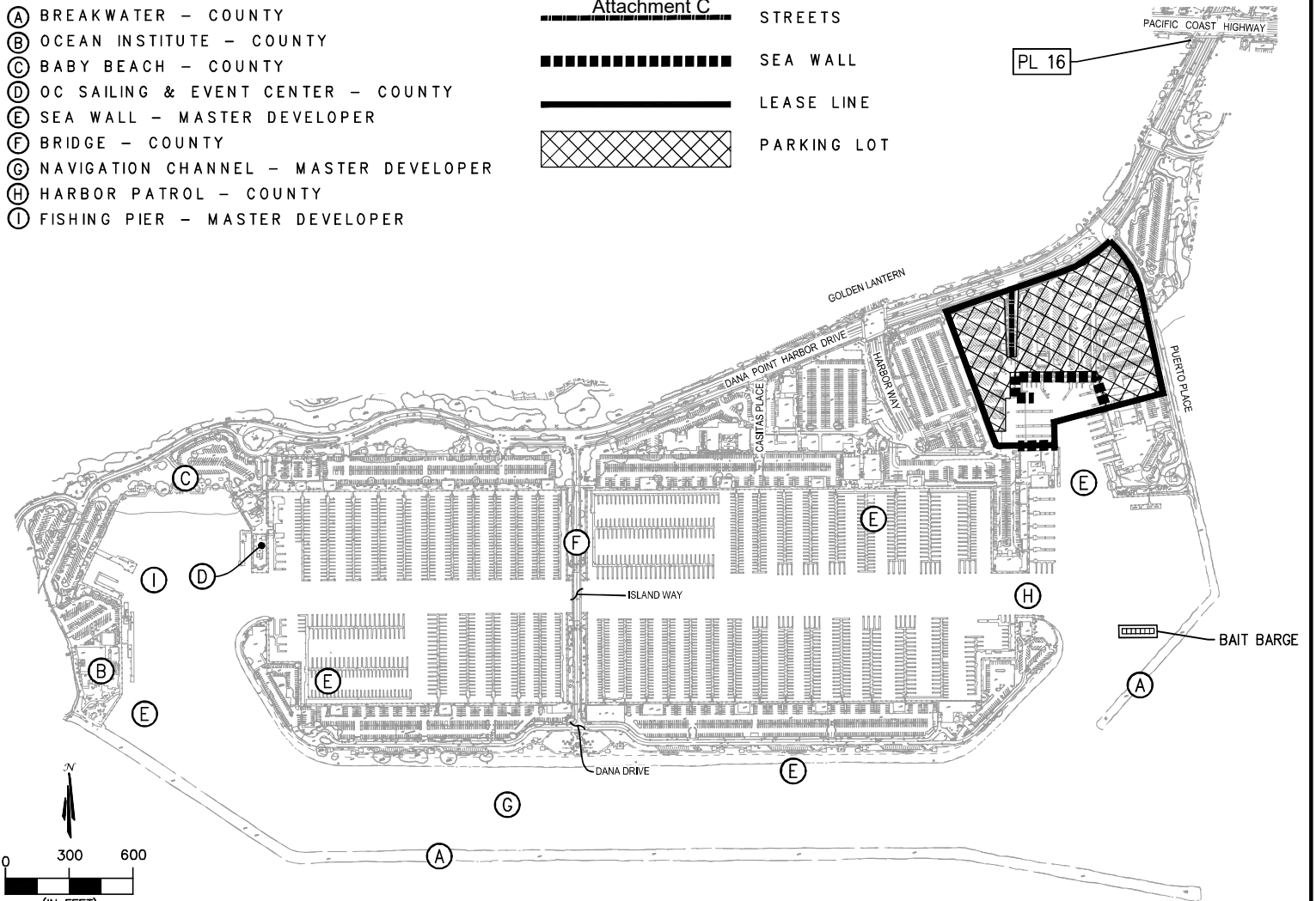
DANA POINT HARBOR DRYSTACK EXHIBIT H DEPICTION OF PROPERTY STRUCTURES Page 166 of 181
