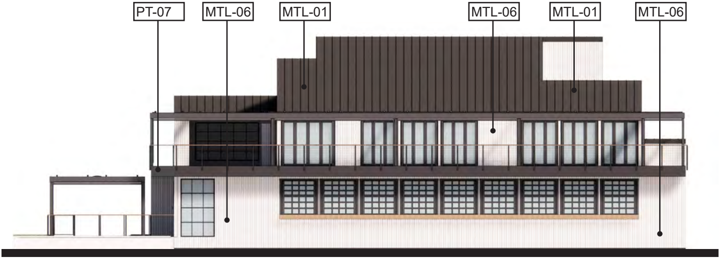
EAST ELEVATION
