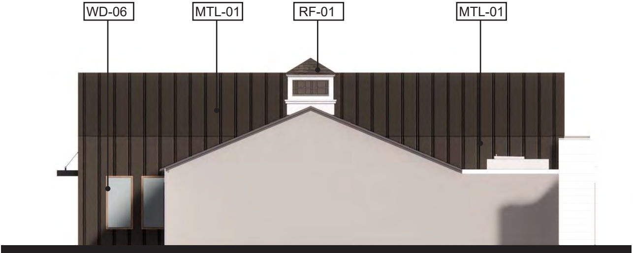
EAST ELEVATION
