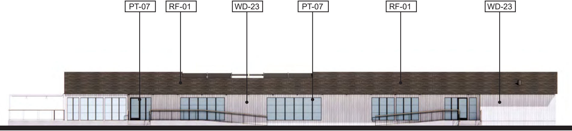
EAST ELEVATION
