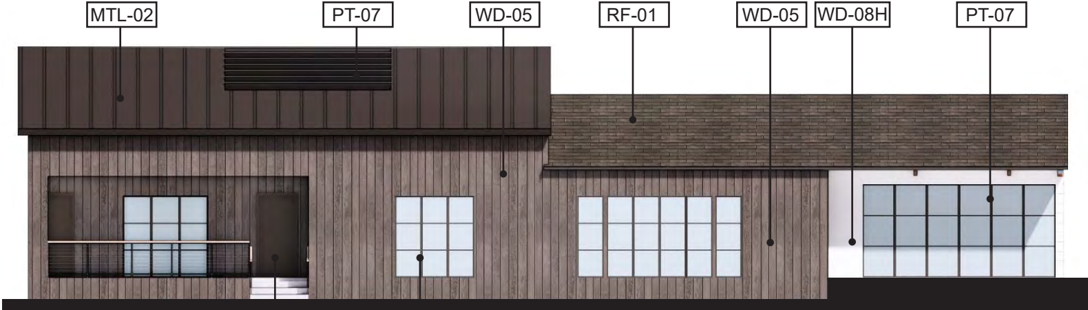
EAST ELEVATION
