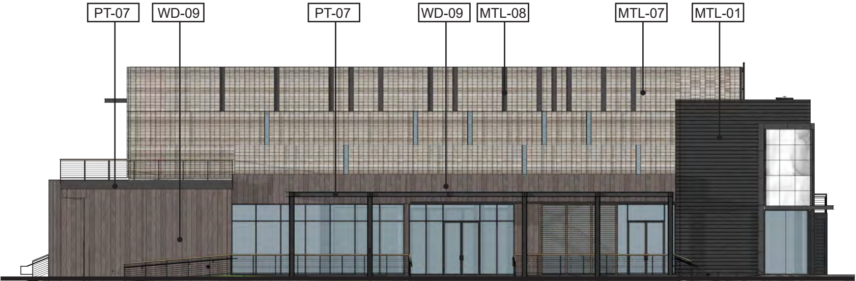
NORTH ELEVATION
