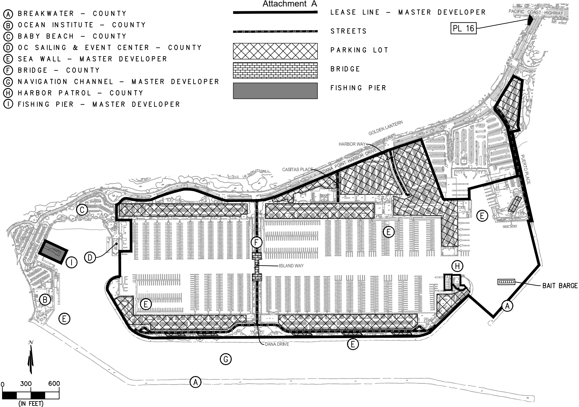
DANA POINT HARBOR EXHIBIT H DEPICTION OF PROPERTY STRUCTURES Page 460 of 467
